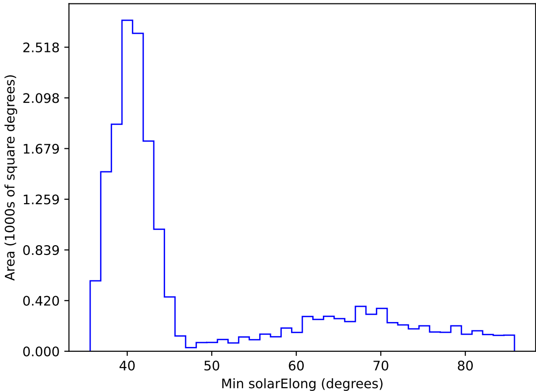
too_elab_r64_d2_griz_v3.4_10yrs WFD i band: Min solarElong
