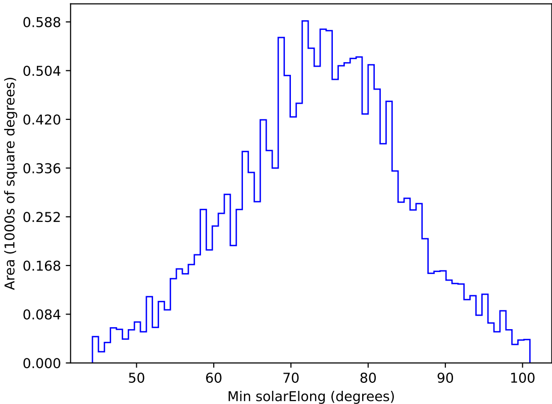
too_elab_r64_d2_griz_v3.4_10yrs WFD g band: Min solarElong
