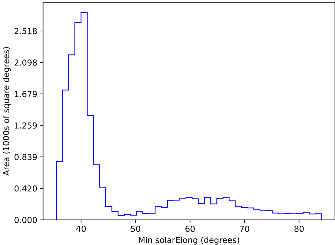
too_elab_r64_d2_griz_v3.4_10yrs WFD all bands: Min solarElong
