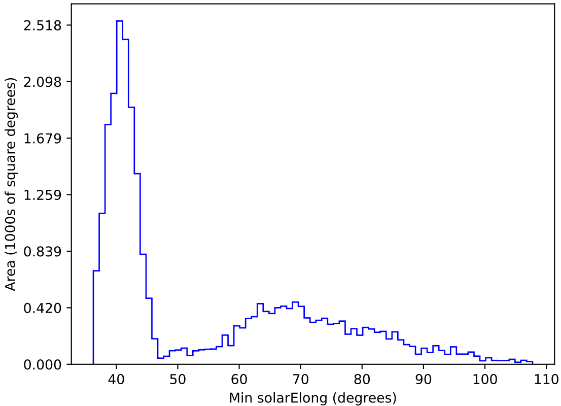
too_elab_r64_d2_griz_v3.4_10yrs All sky z band: Min solarElong
