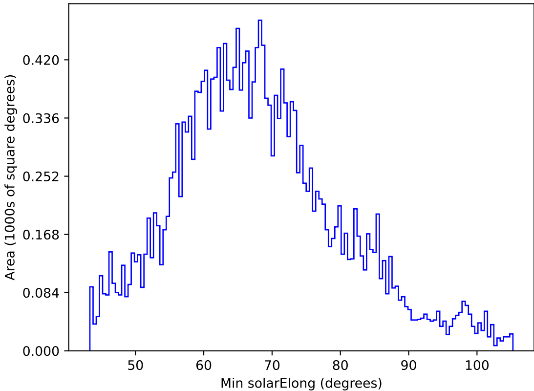
too_elab_r64_d2_griz_v3.4_10yrs All sky y band: Min solarElong
