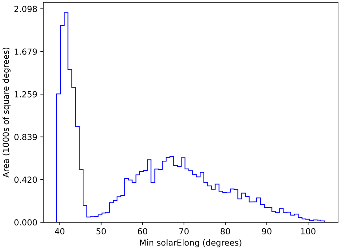
too_elab_r64_d2_griz_v3.4_10yrs All sky r band: Min solarElong
