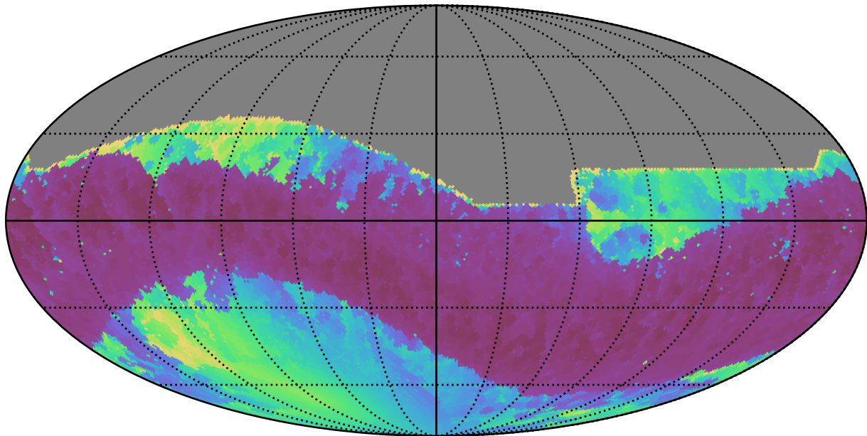
too_elab_r64_d2_griz_v3.4_10yrs All sky i band: Min solarElong
