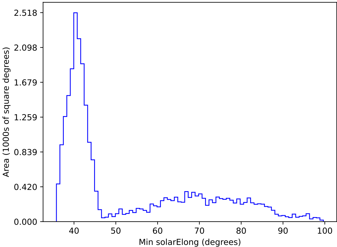
too_elab_r64_d2_griz_v3.4_10yrs All sky i band: Min solarElong
