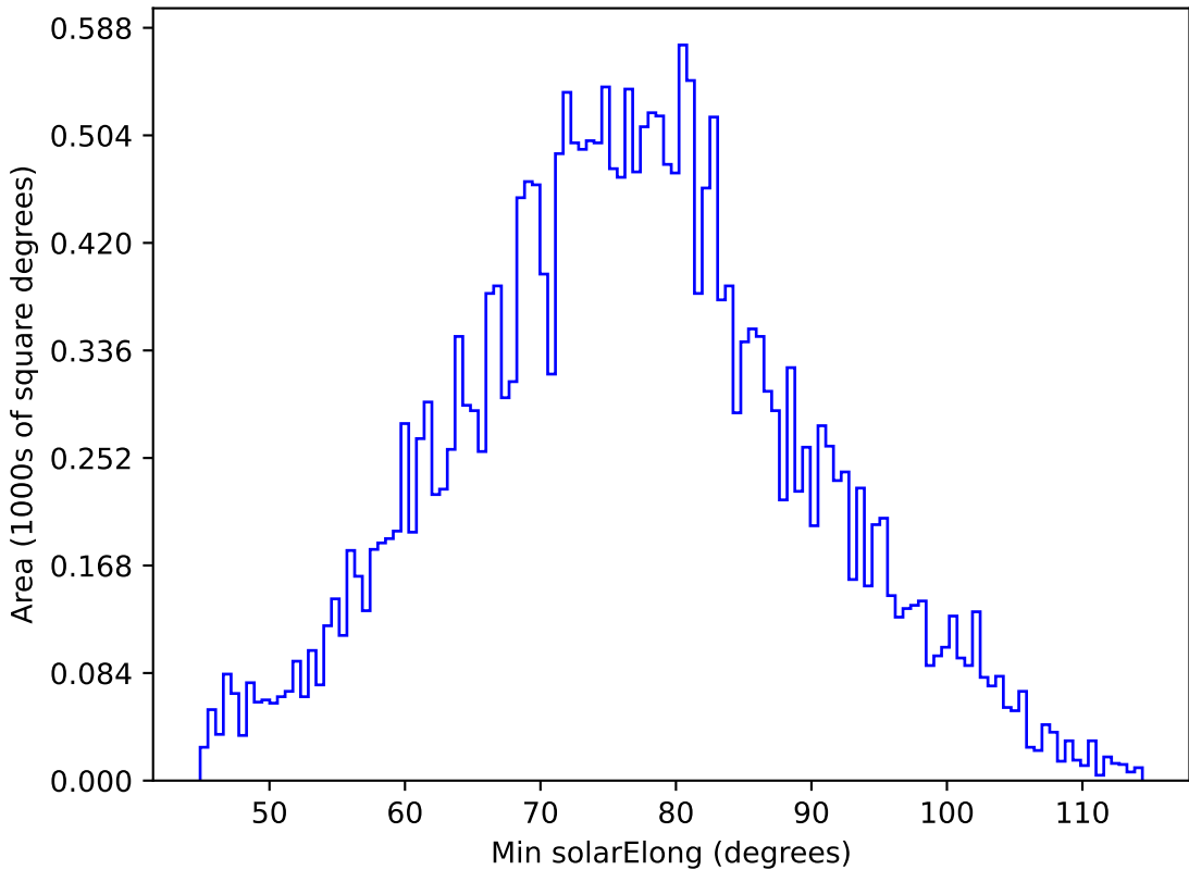
too_elab_r64_d2_griz_v3.4_10yrs All sky g band: Min solarElong
