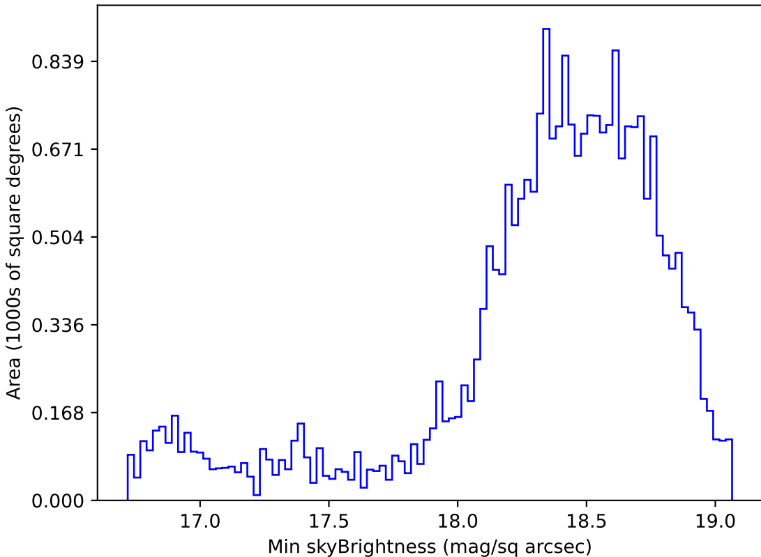
too_elab_r64_d2_griz_v3.4_10yrs Yr 1 z band: Min skyBrightness
