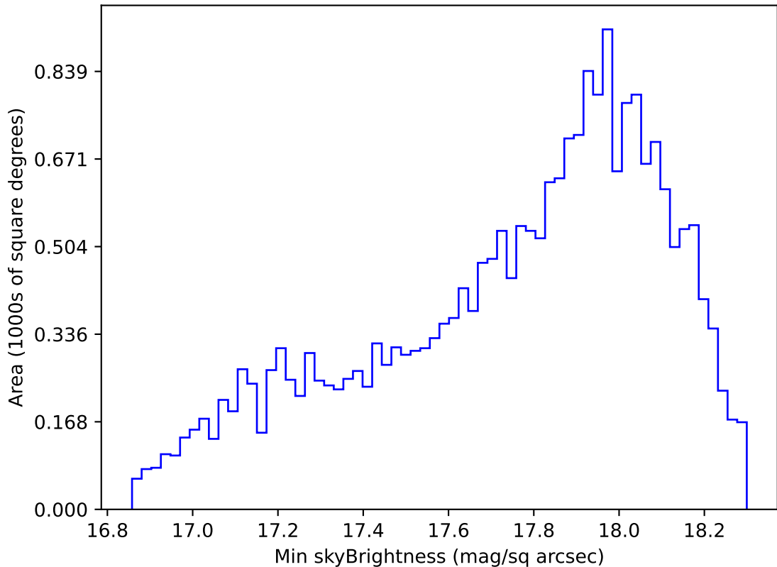
too_elab_r64_d2_griz_v3.4_10yrs Yr 1 y band: Min skyBrightness
