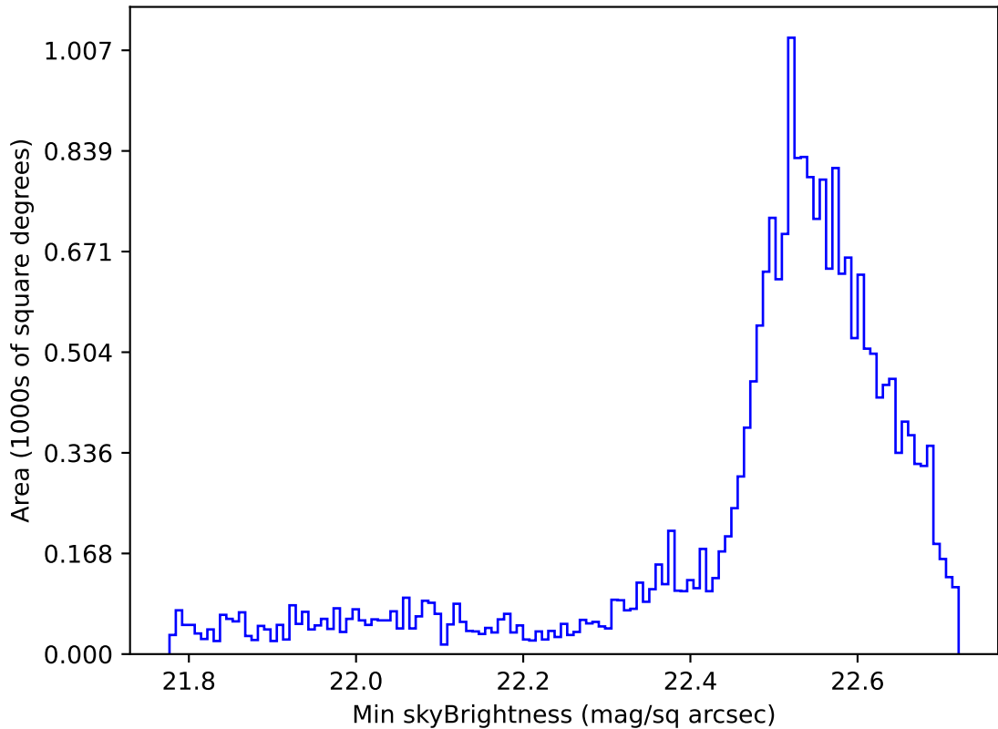
too_elab_r64_d2_griz_v3.4_10yrs Yr 1 u band: Min skyBrightness
