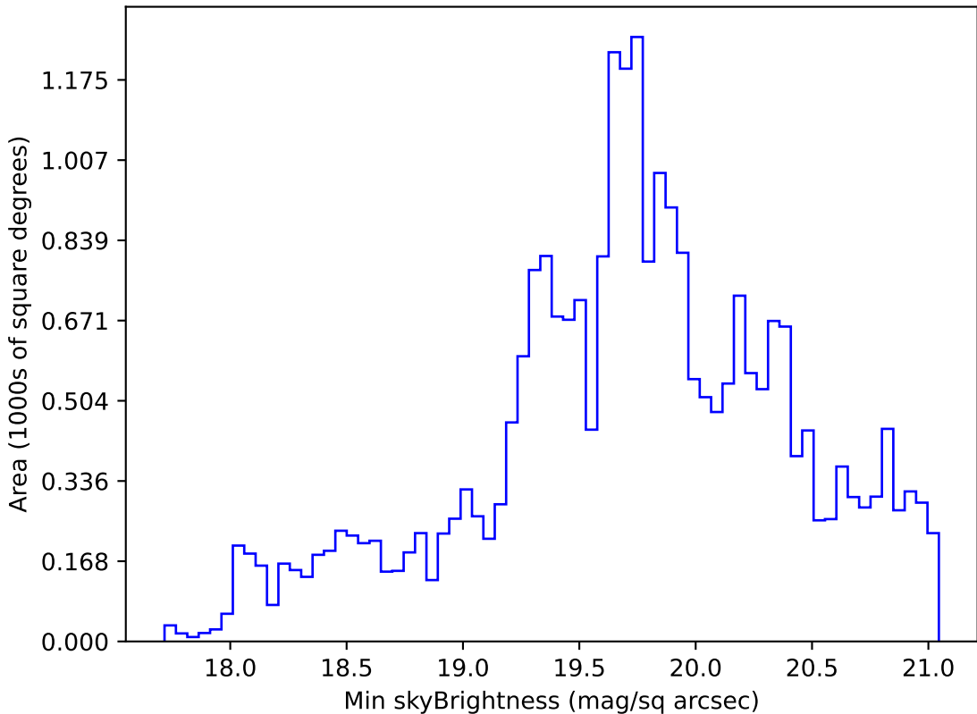
too_elab_r64_d2_griz_v3.4_10yrs Yr 1 r band: Min skyBrightness
