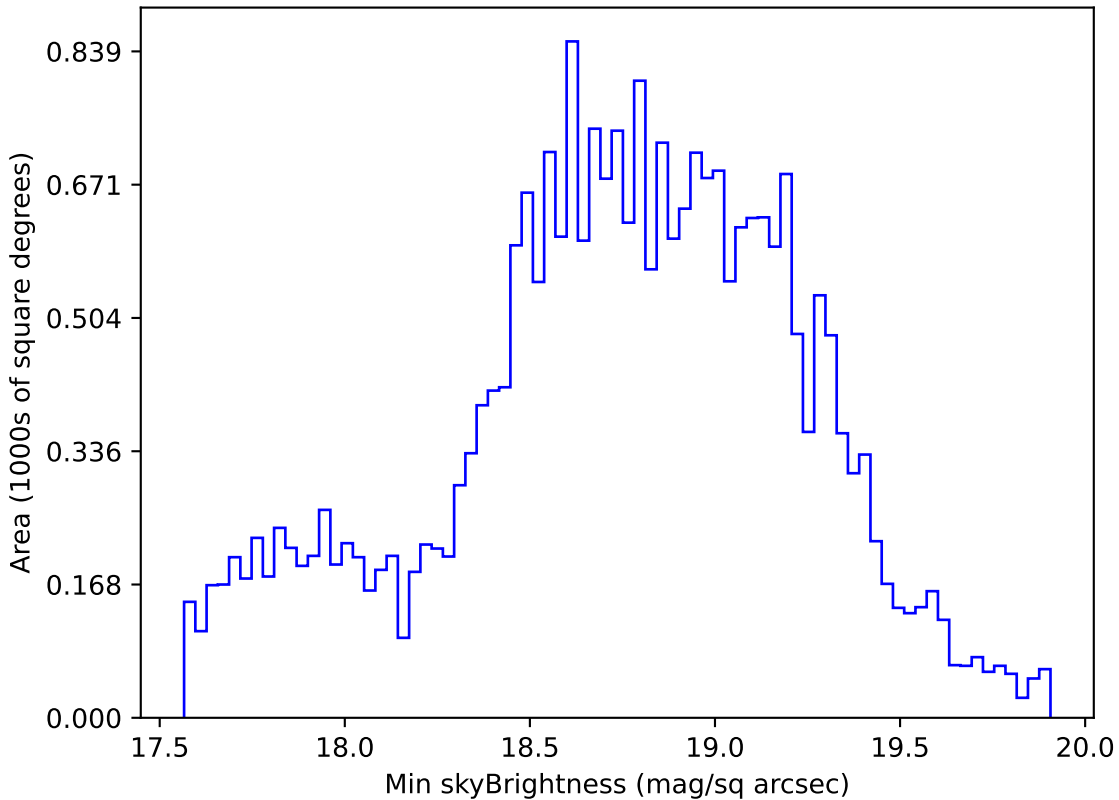
too_elab_r64_d2_griz_v3.4_10yrs Yr 1 i band: Min skyBrightness
