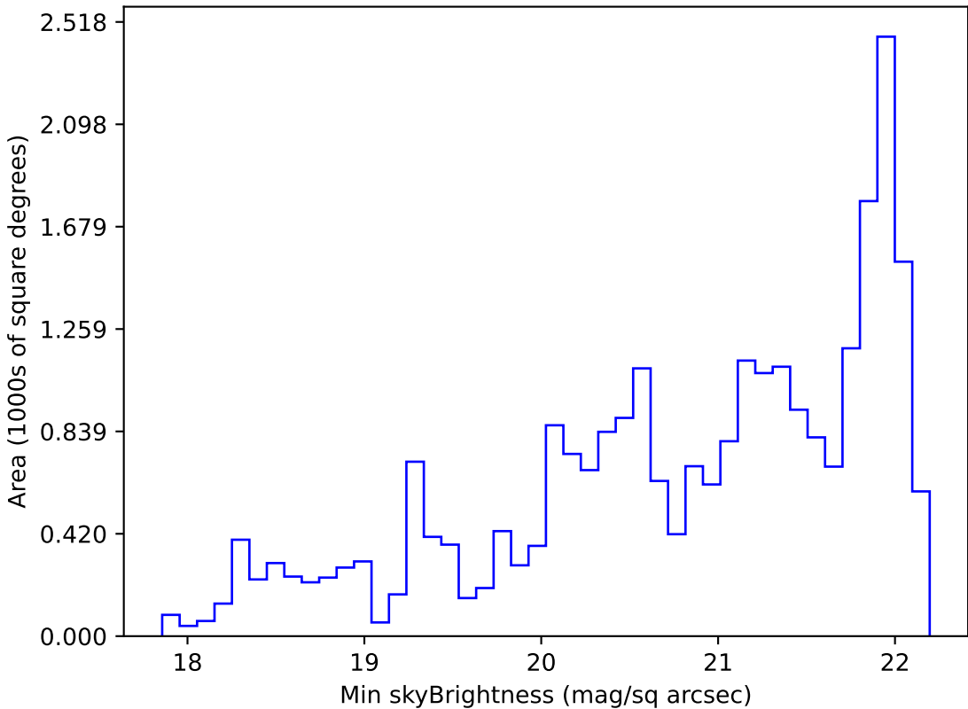
too_elab_r64_d2_griz_v3.4_10yrs Yr 1 g band: Min skyBrightness
