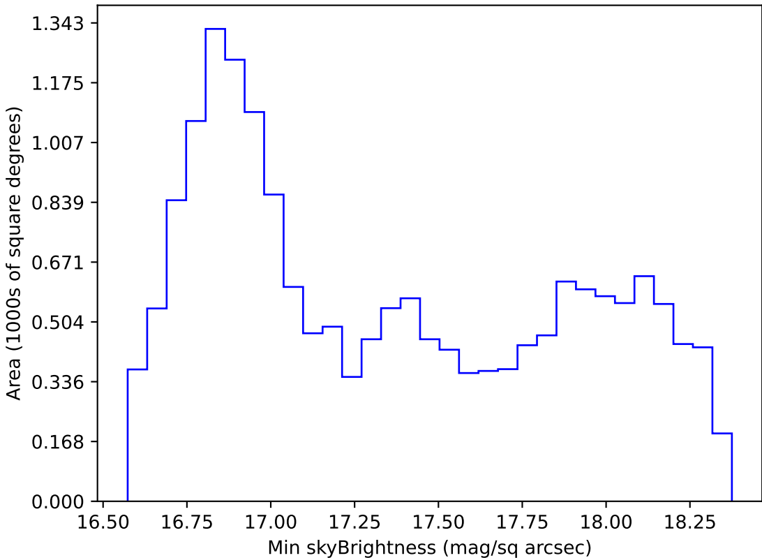
too_elab_r64_d2_griz_v3.4_10yrs WFD z band: Min skyBrightness
