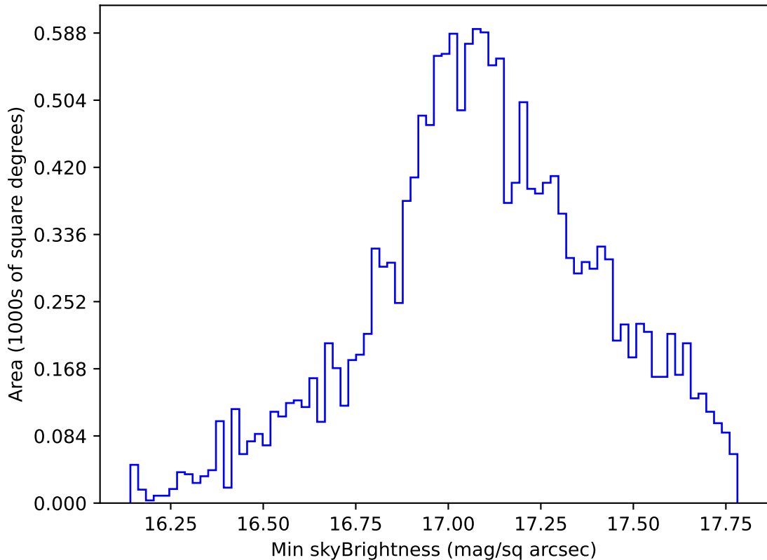
too_elab_r64_d2_griz_v3.4_10yrs WFD y band: Min skyBrightness
