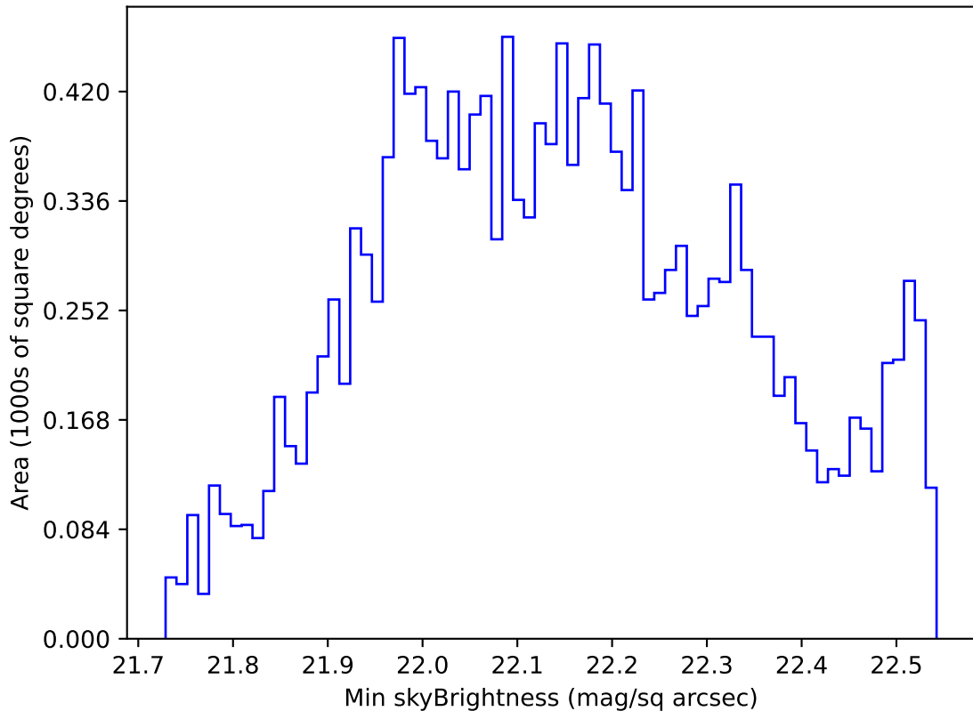
too_elab_r64_d2_griz_v3.4_10yrs WFD u band: Min skyBrightness
