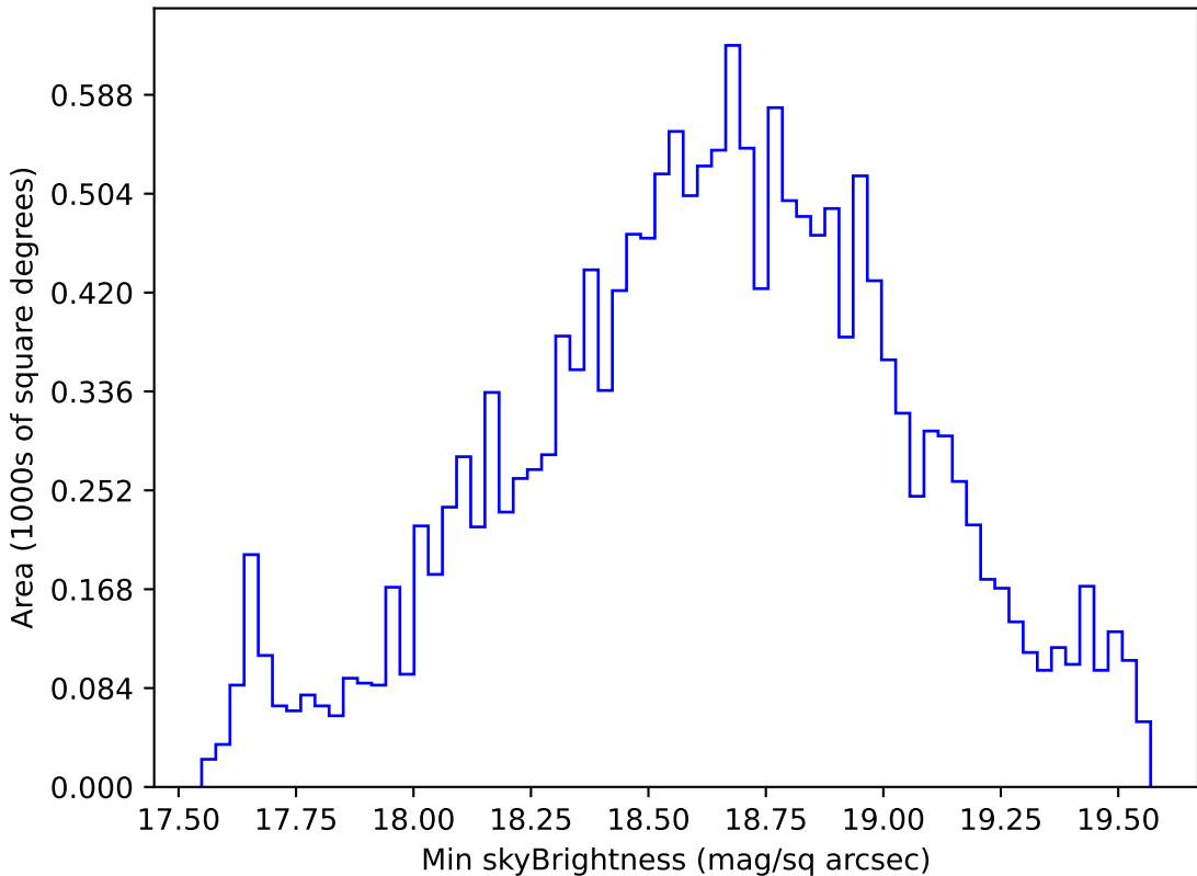
too_elab_r64_d2_griz_v3.4_10yrs WFD r band: Min skyBrightness
