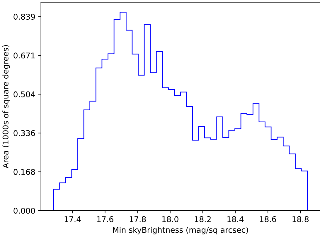
too_elab_r64_d2_griz_v3.4_10yrs WFD i band: Min skyBrightness
