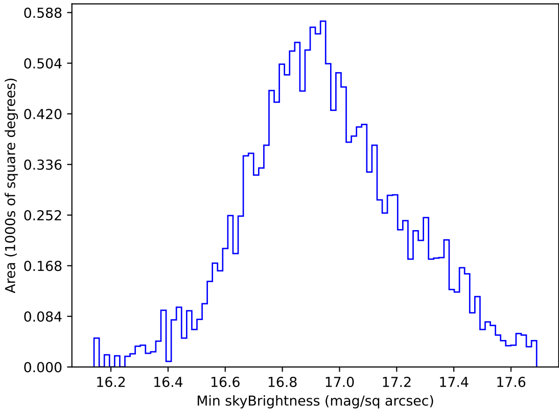
too_elab_r64_d2_griz_v3.4_10yrs WFD all bands: Min skyBrightness
