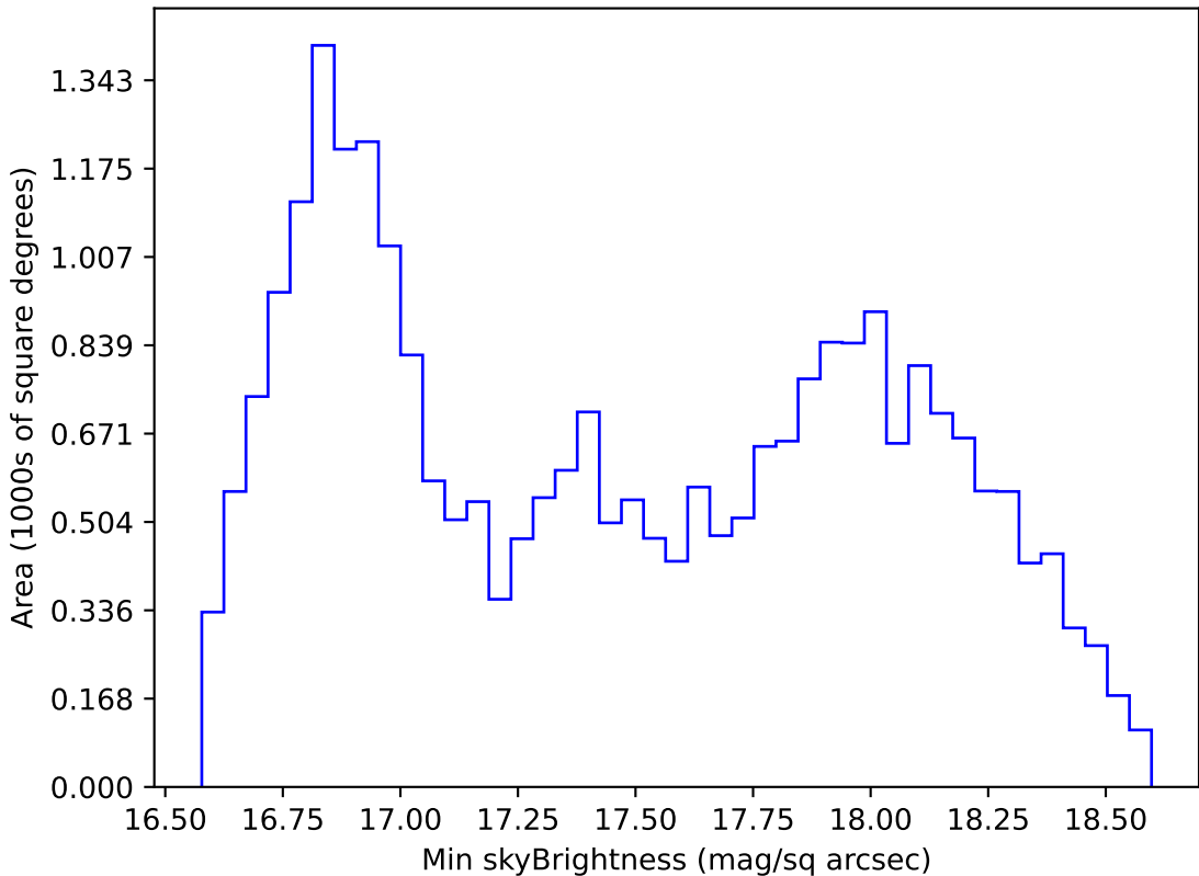
too_elab_r64_d2_griz_v3.4_10yrs All sky z band: Min skyBrightness
