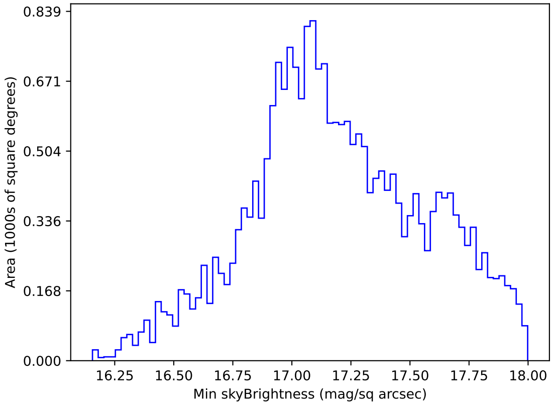
too_elab_r64_d2_griz_v3.4_10yrs All sky y band: Min skyBrightness
