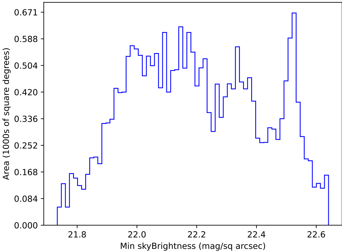
too_elab_r64_d2_griz_v3.4_10yrs All sky u band: Min skyBrightness
