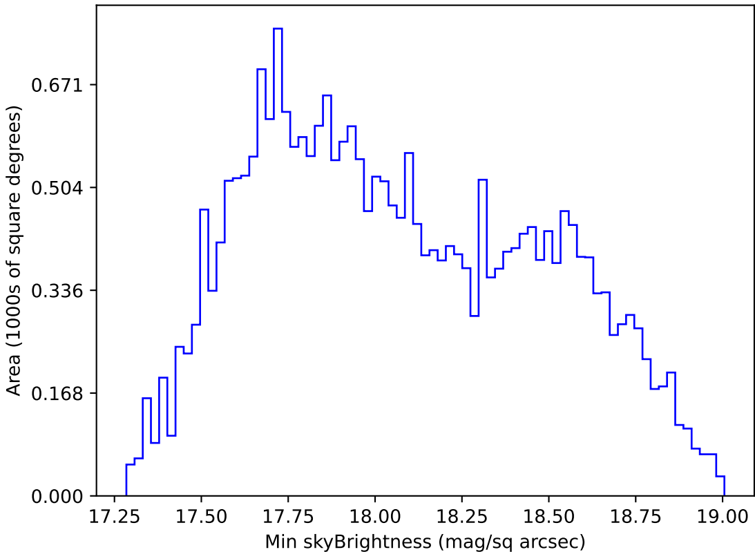
too_elab_r64_d2_griz_v3.4_10yrs All sky i band: Min skyBrightness
