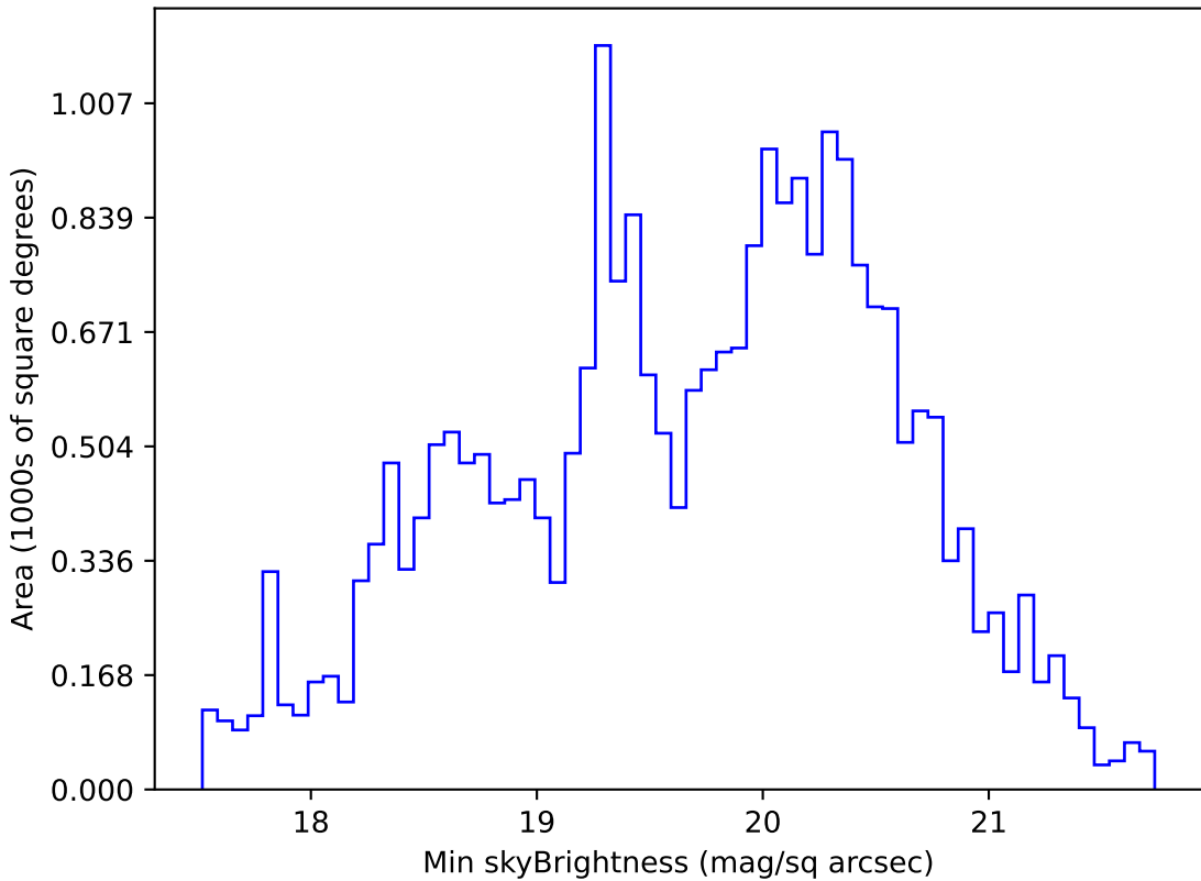
too_elab_r64_d2_griz_v3.4_10yrs All sky g band: Min skyBrightness
