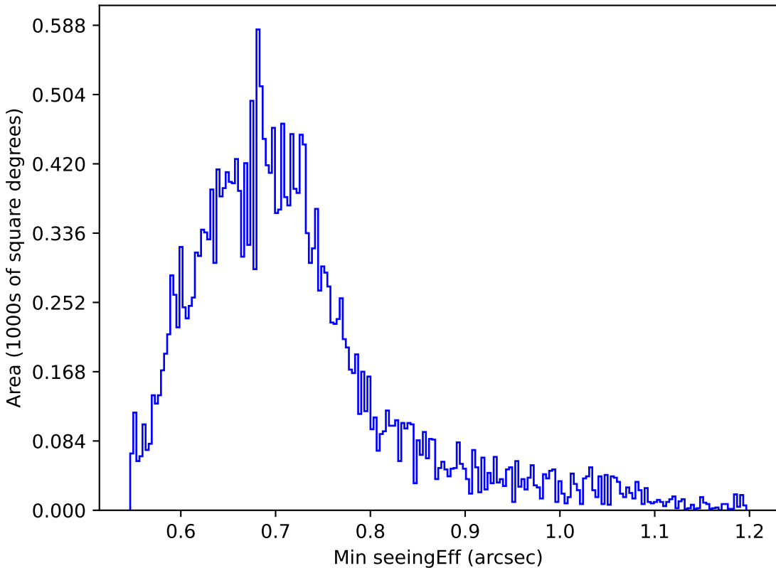
too_elab_r64_d2_griz_v3.4_10yrs Yr 1 z band: Min seeingEff
