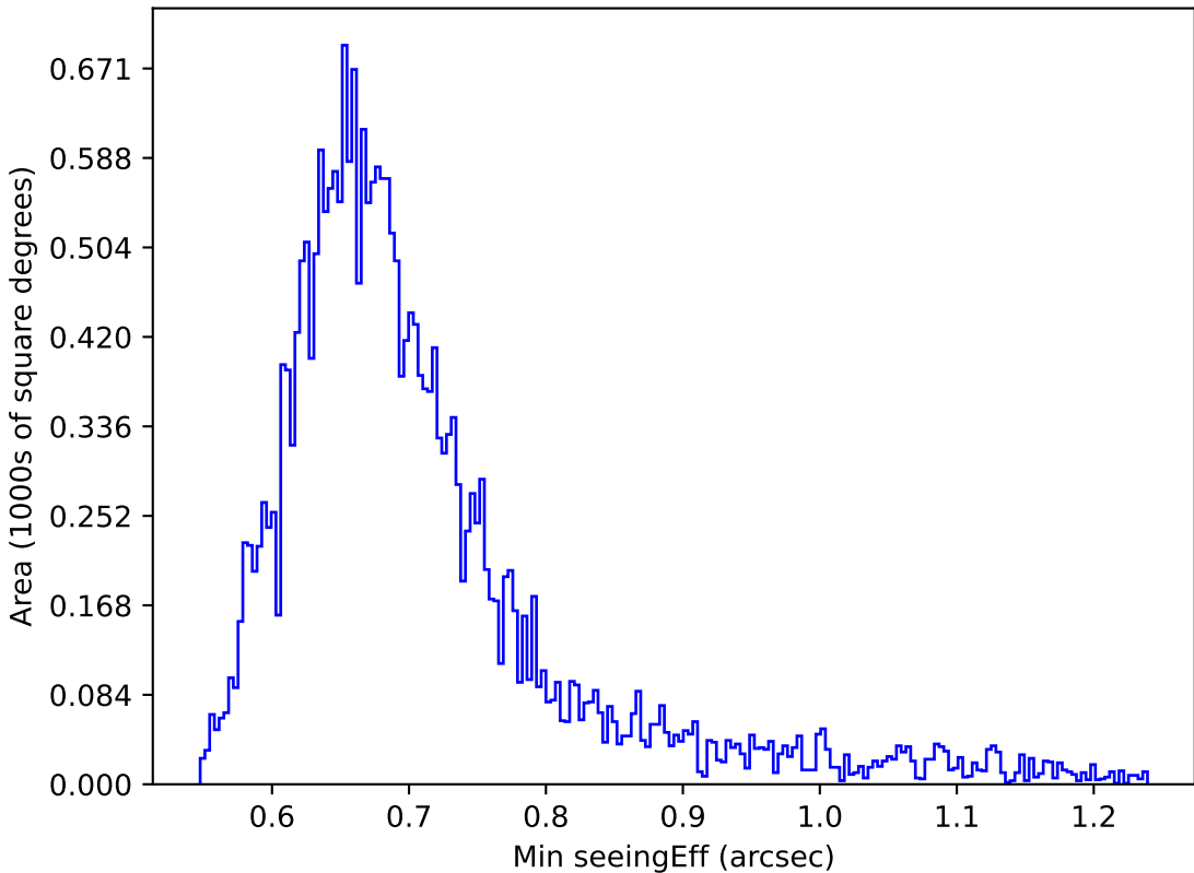
too_elab_r64_d2_griz_v3.4_10yrs Yr 1 i band: Min seeingEff
