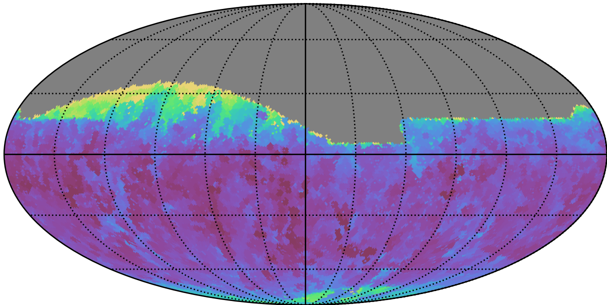
too_elab_r64_d2_griz_v3.4_10yrs Yr 1 all bands: Min seeingEff
