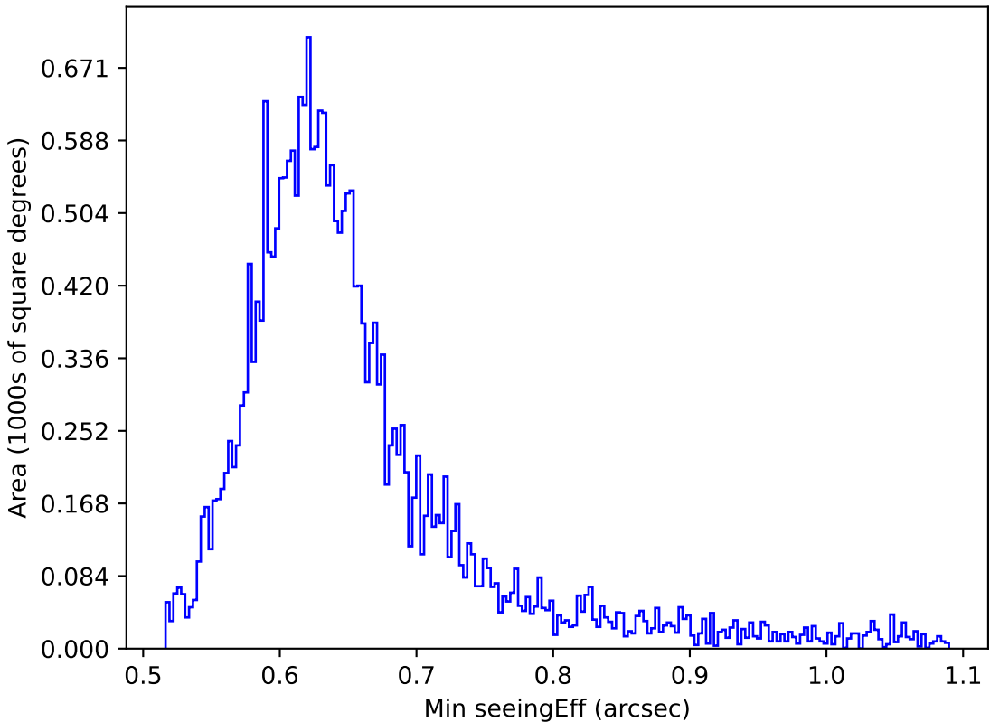
too_elab_r64_d2_griz_v3.4_10yrs Yr 1 all bands: Min seeingEff
