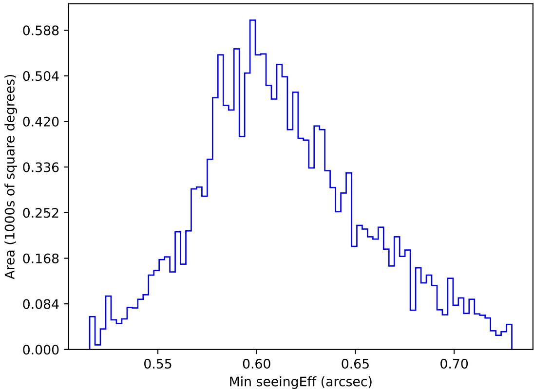
too_elab_r64_d2_griz_v3.4_10yrs WFD z band: Min seeingEff
