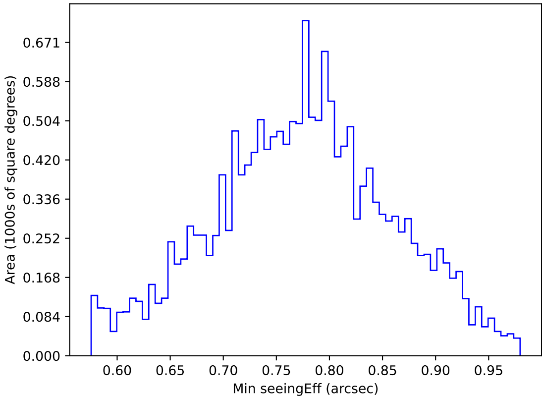
too_elab_r64_d2_griz_v3.4_10yrs WFD u band: Min seeingEff
