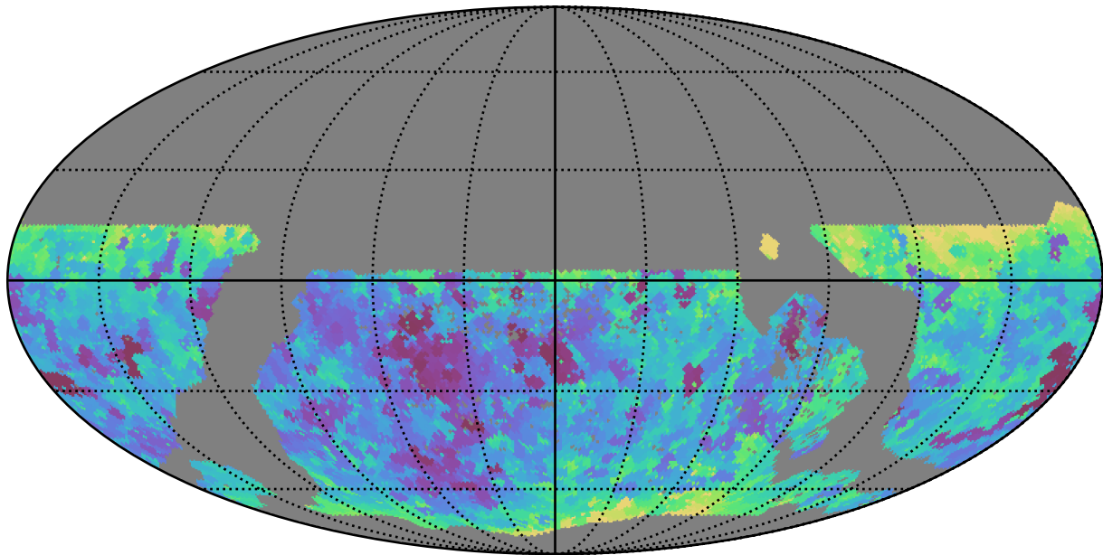
too_elab_r64_d2_griz_v3.4_10yrs WFD r band: Min seeingEff
