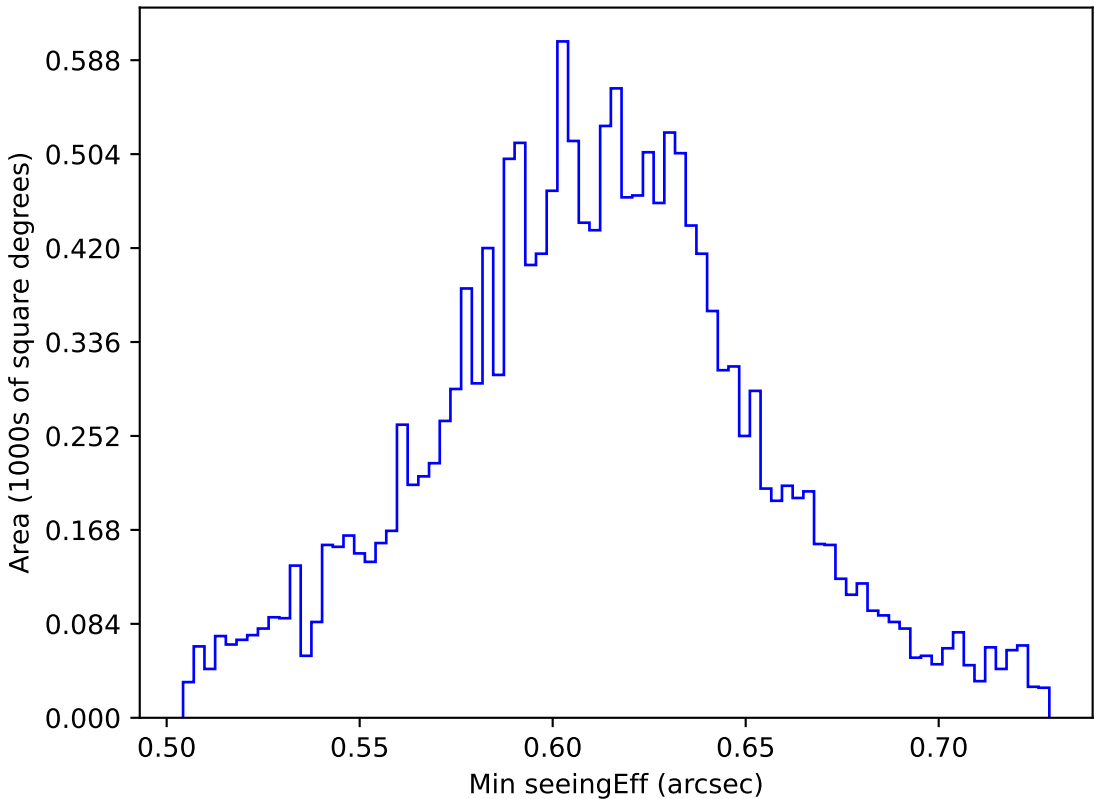
too_elab_r64_d2_griz_v3.4_10yrs WFD r band: Min seeingEff
