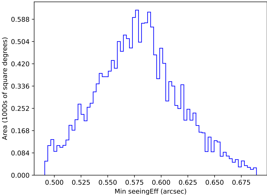
too_elab_r64_d2_griz_v3.4_10yrs WFD all bands: Min seeingEff
