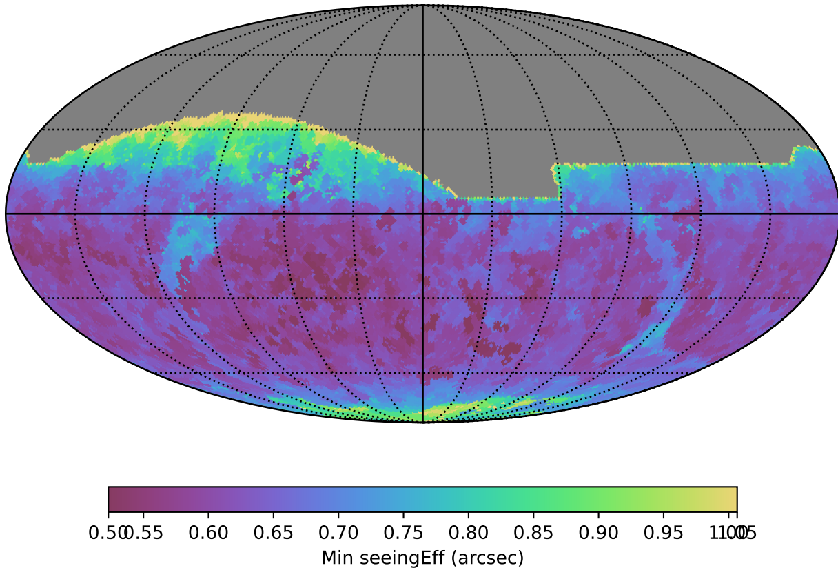
too_elab_r64_d2_griz_v3.4_10yrs All sky z band: Min seeingEff
