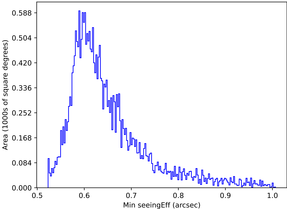
too_elab_r64_d2_griz_v3.4_10yrs All sky z band: Min seeingEff
