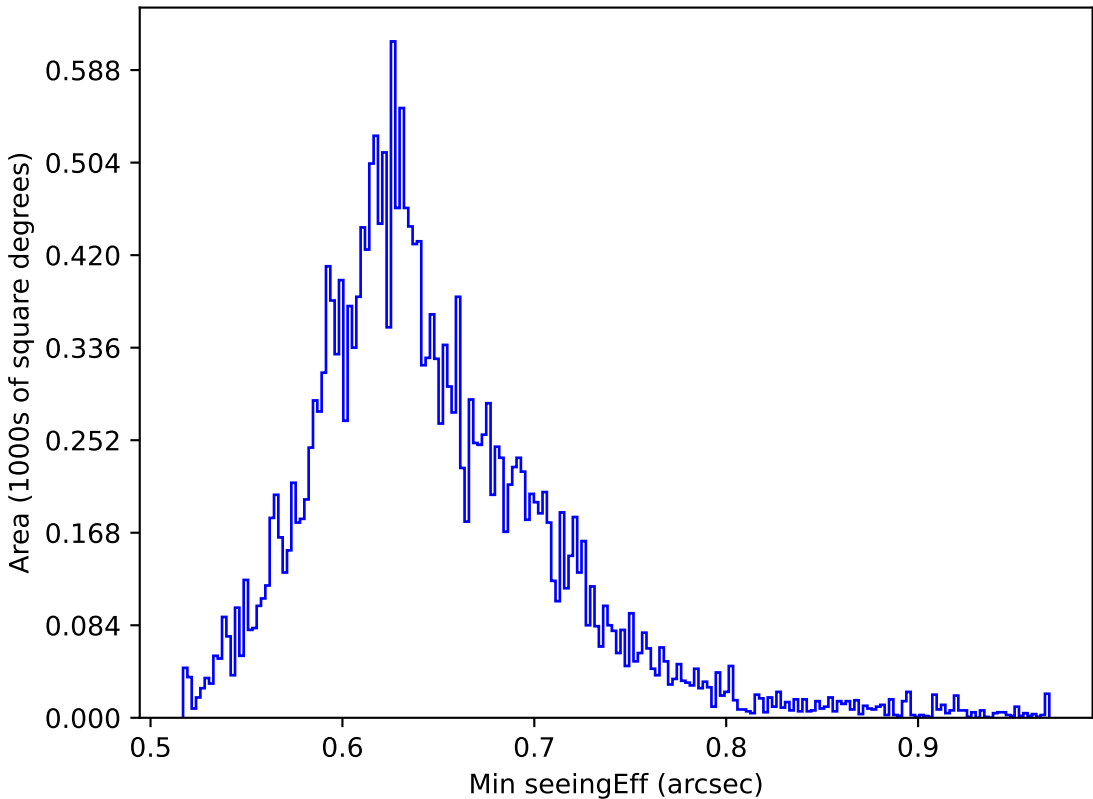
too_elab_r64_d2_griz_v3.4_10yrs All sky y band: Min seeingEff
