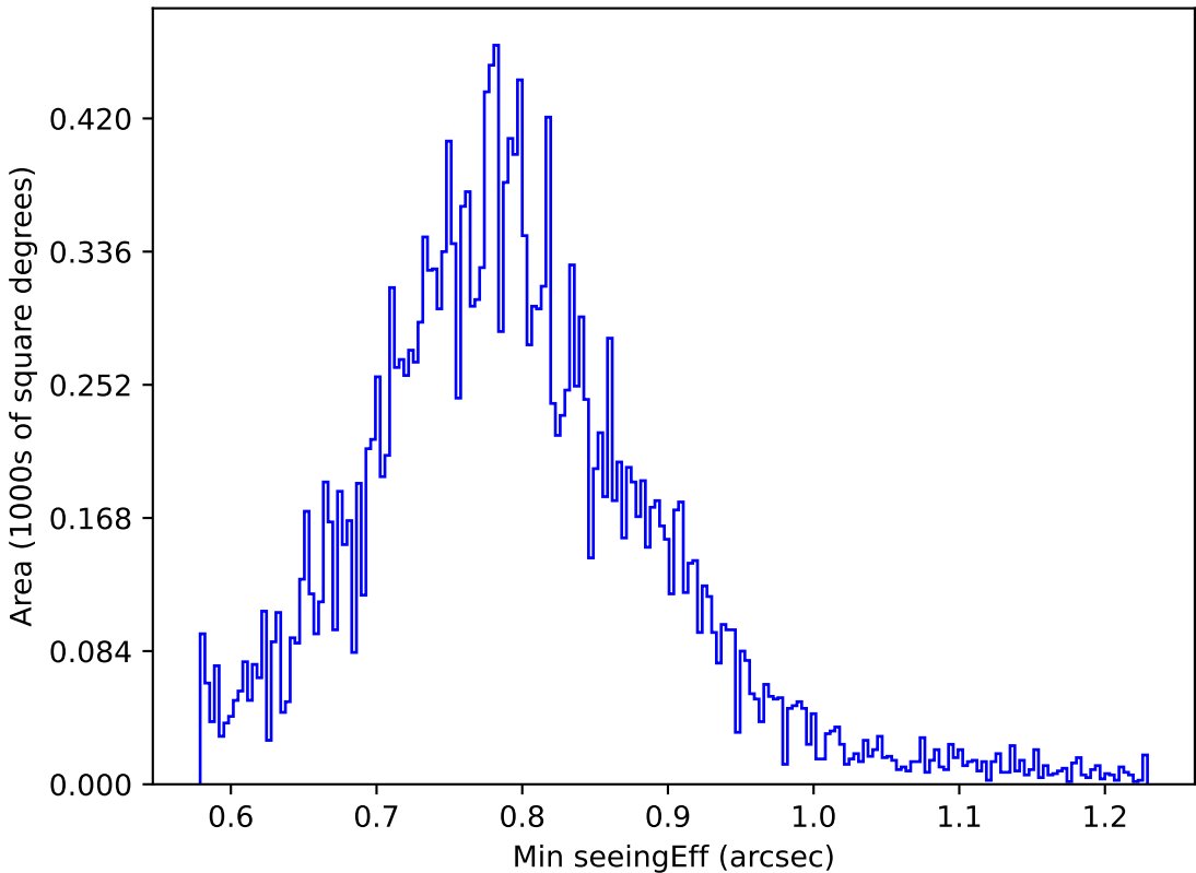
too_elab_r64_d2_griz_v3.4_10yrs All sky u band: Min seeingEff
