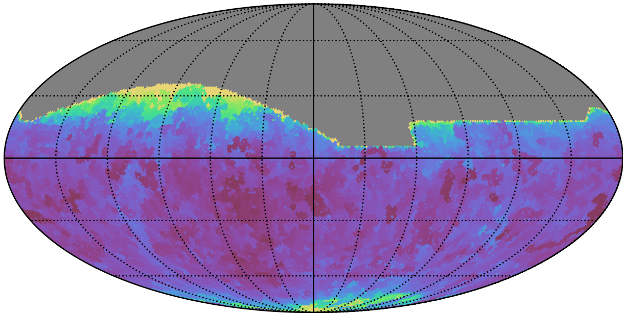
too_elab_r64_d2_griz_v3.4_10yrs All sky r band: Min seeingEff
