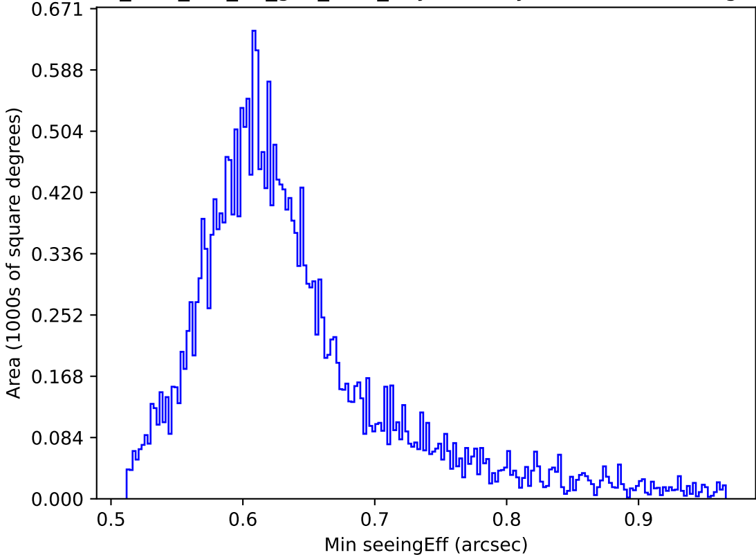
too_elab_r64_d2_griz_v3.4_10yrs All sky i band: Min seeingEff
