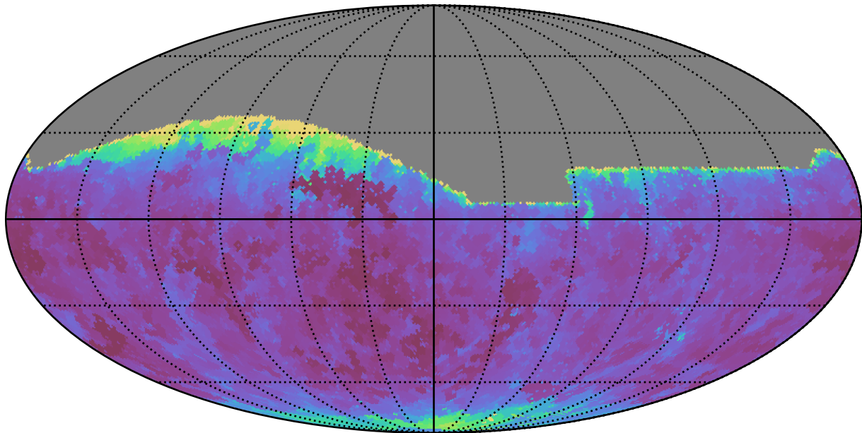
too_elab_r64_d2_griz_v3.4_10yrs All sky g band: Min seeingEff
