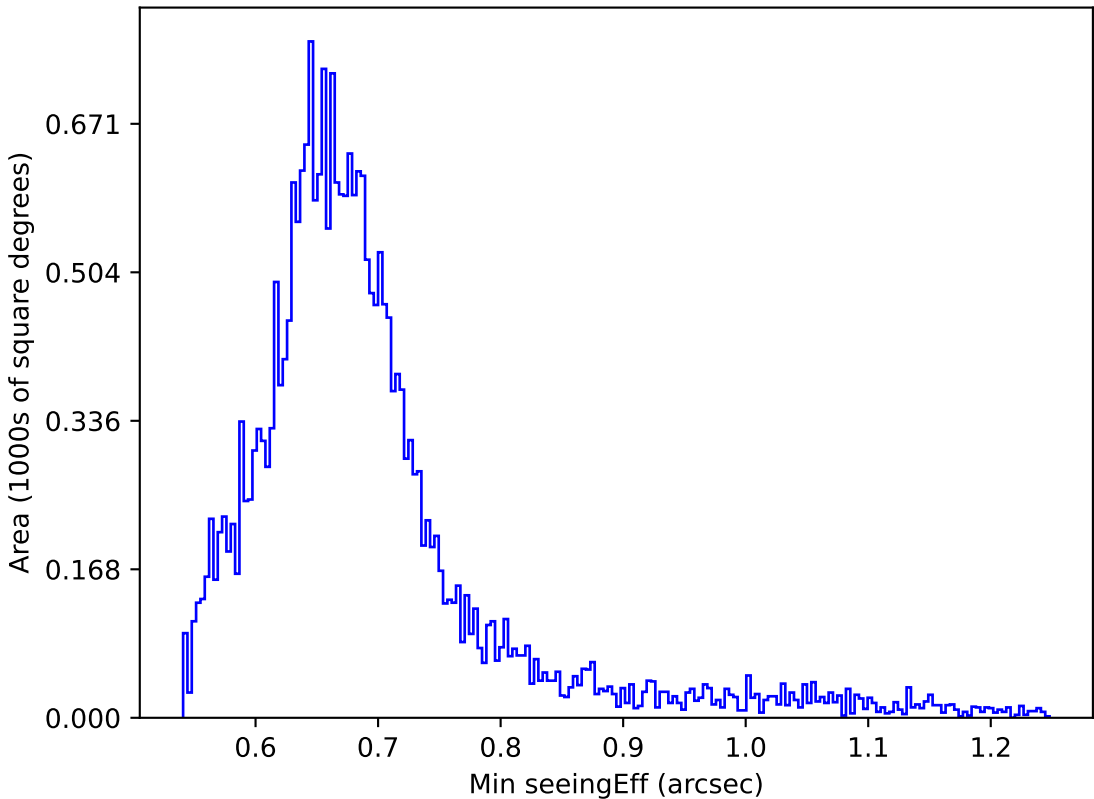
too_elab_r64_d2_griz_v3.4_10yrs All sky g band: Min seeingEff
