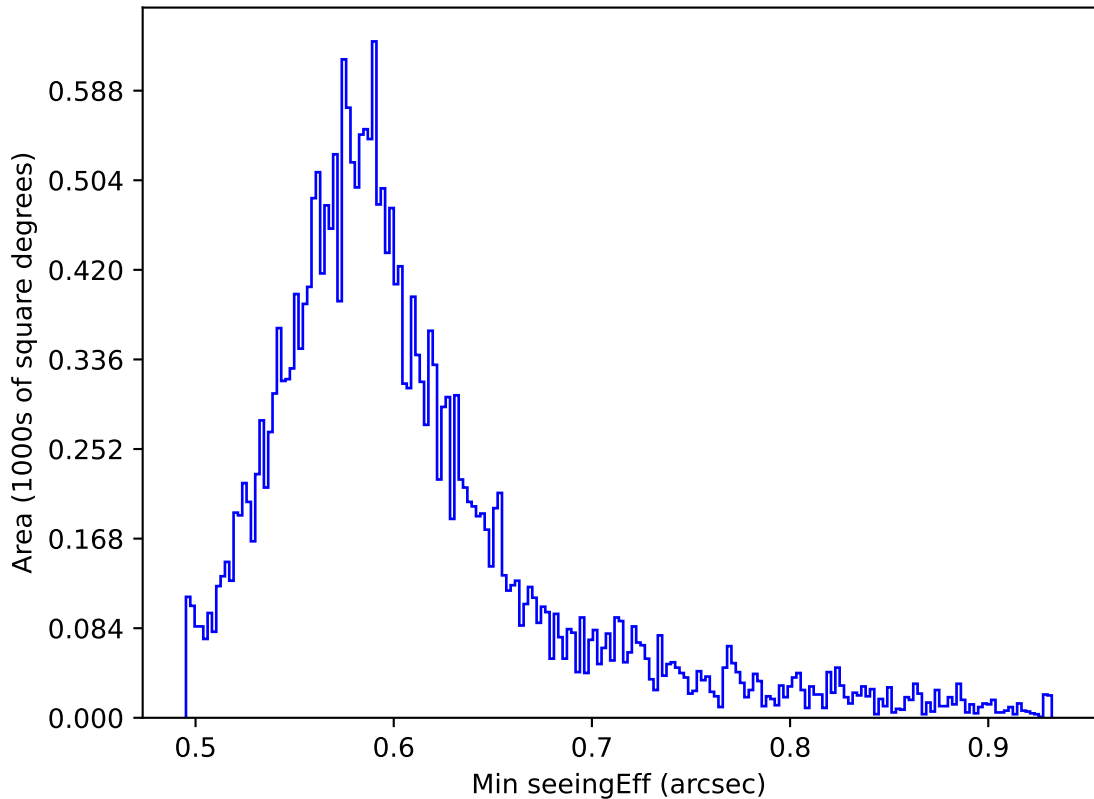
too_elab_r64_d2_griz_v3.4_10yrs All sky all bands: Min seeingEff
