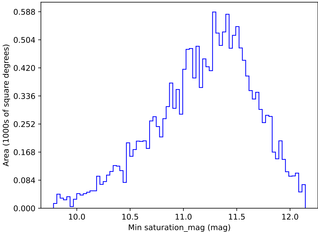
too_elab_r64_d2_griz_v3.4_10yrs WFD y band: Min saturation_mag
