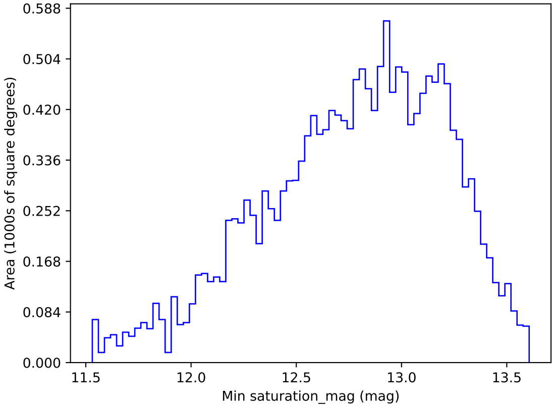
too_elab_r64_d2_griz_v3.4_10yrs WFD g band: Min saturation_mag
