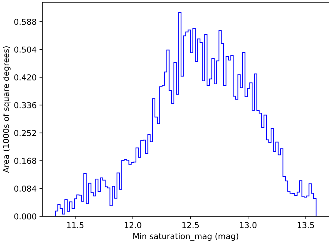
too_elab_r64_d2_griz_v3.4_10yrs All sky r band: Min saturation_mag
