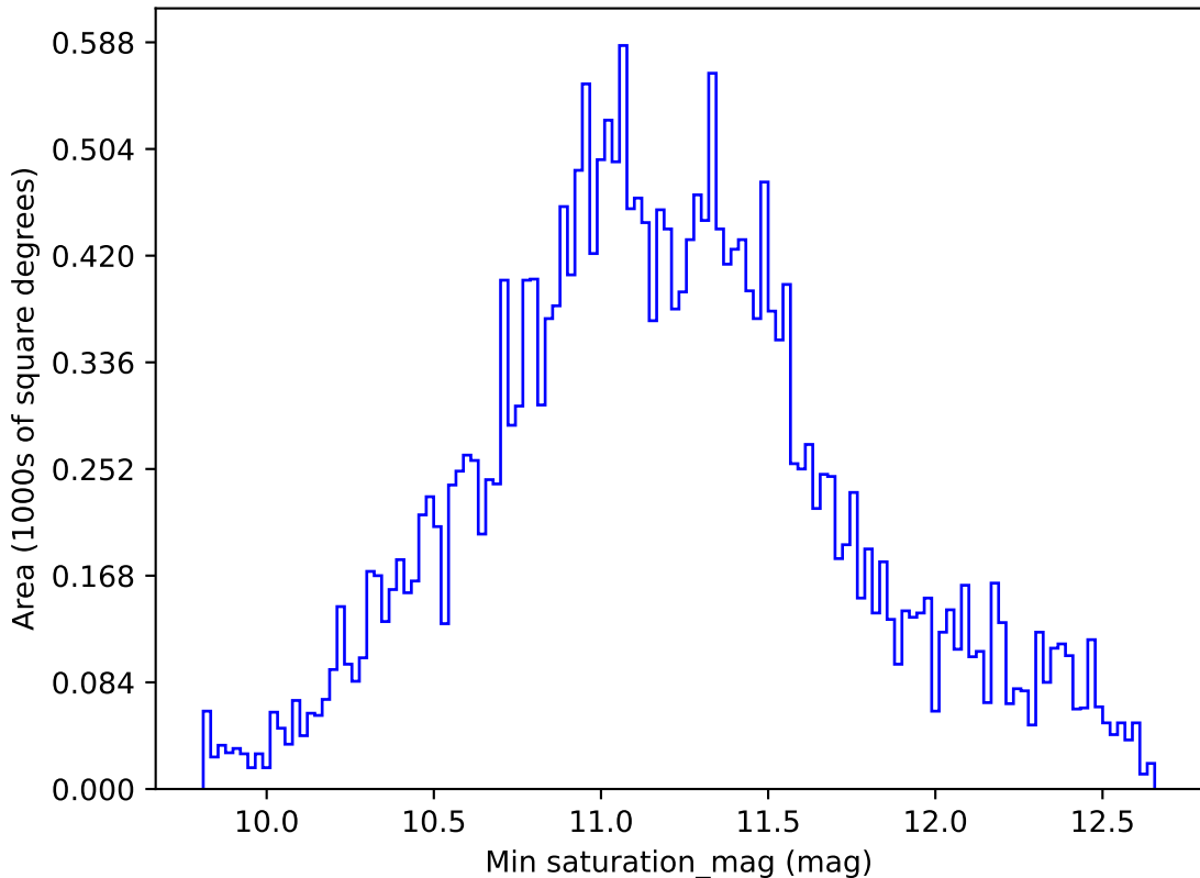
too_elab_r64_d2_griz_v3.4_10yrs All sky all bands: Min saturation_mag
