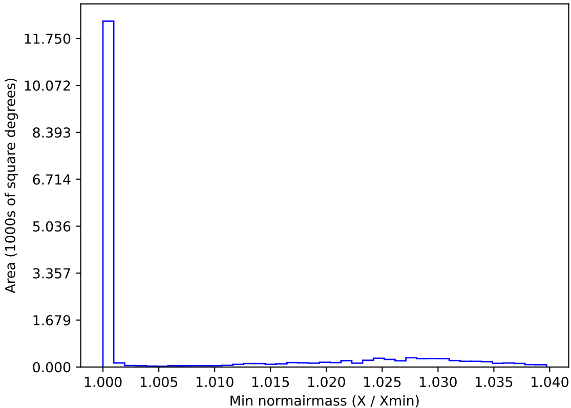
too_elab_r64_d2_griz_v3.4_10yrs WFD y band: Min normairmass
