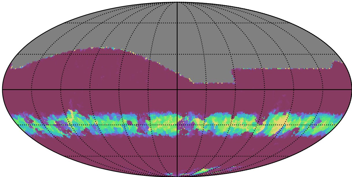
too_elab_r64_d2_griz_v3.4_10yrs All sky r band: Min normairmass
